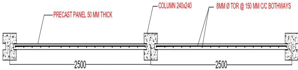
SECTION AT A-B
