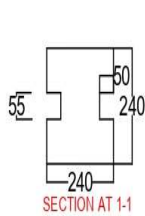
SECTION AT 1-1
