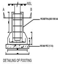
DETAILING OF FOOTING
