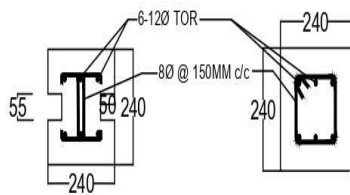
REINFORCEMENT DETAILING OF COLUMN
