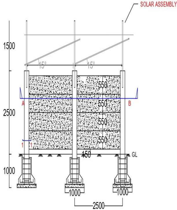
TYPICAL PLAN OF THE PRECAST BOUNDARY WALL
